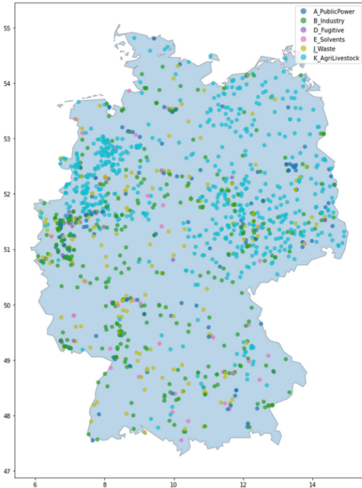
Figure 1: Large Point Sources for different GNFR sectors for Germany for the year 2018 (according to own presentation)
