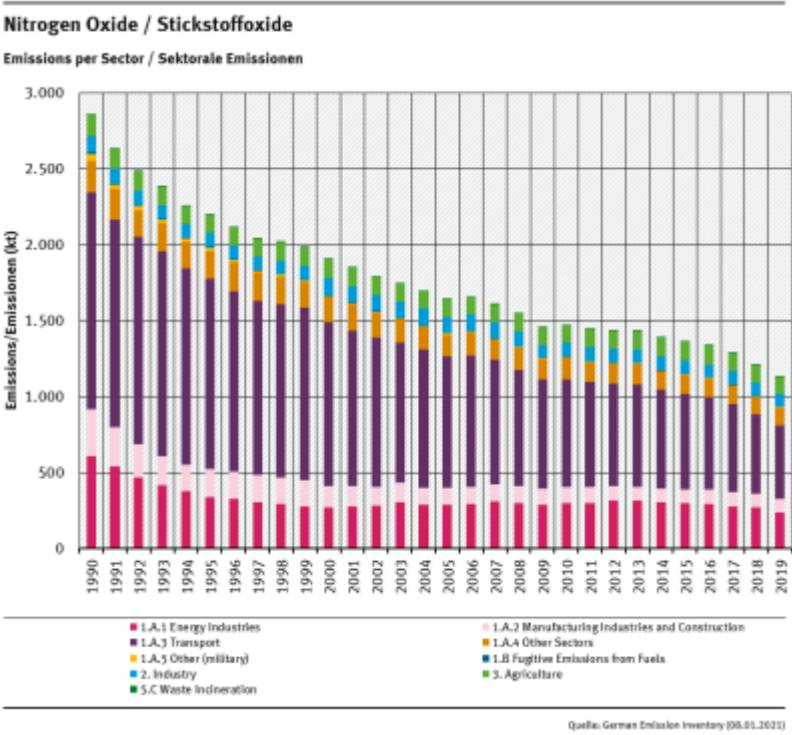
NO x trend by sector
