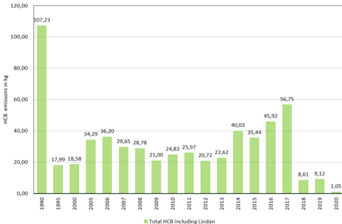
Picture 1: Annual trend of HCB emissions in Germany in the sector agriculture, in kg
