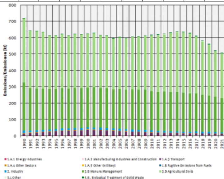
NH 3 trend by sector
