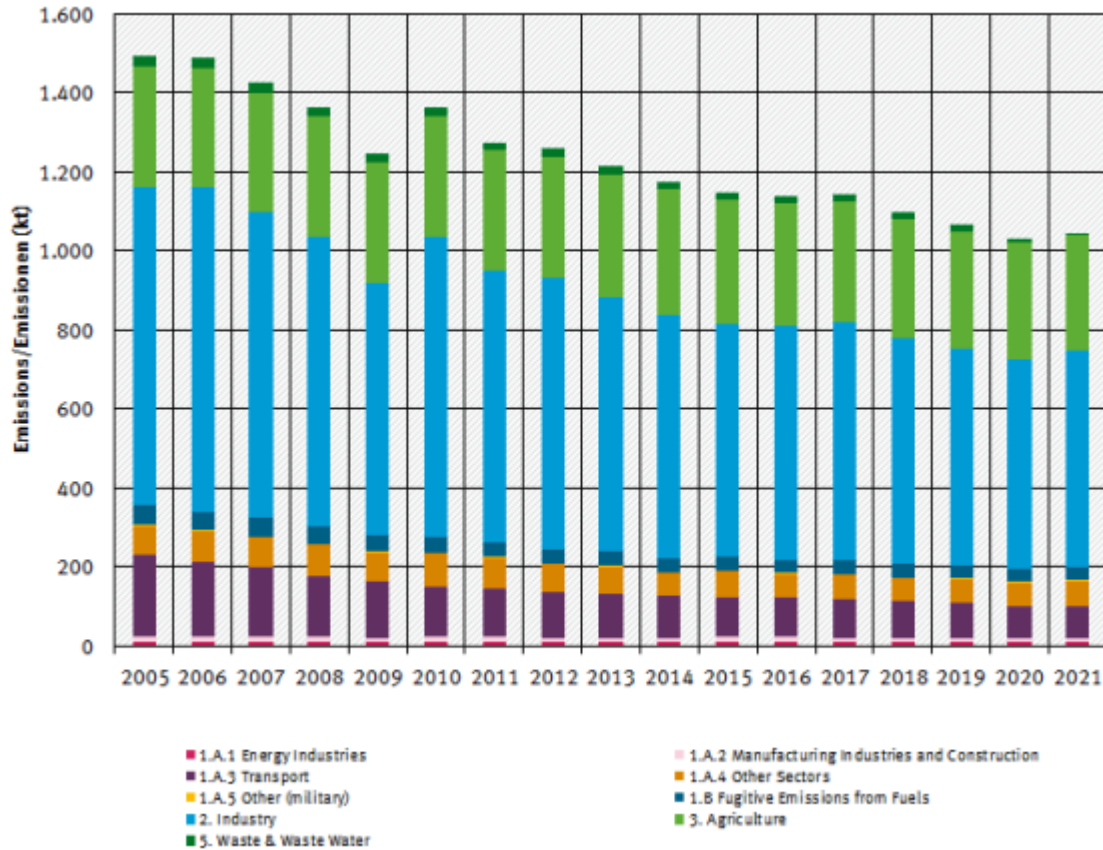
NMVOC trend by sector, from 2005
