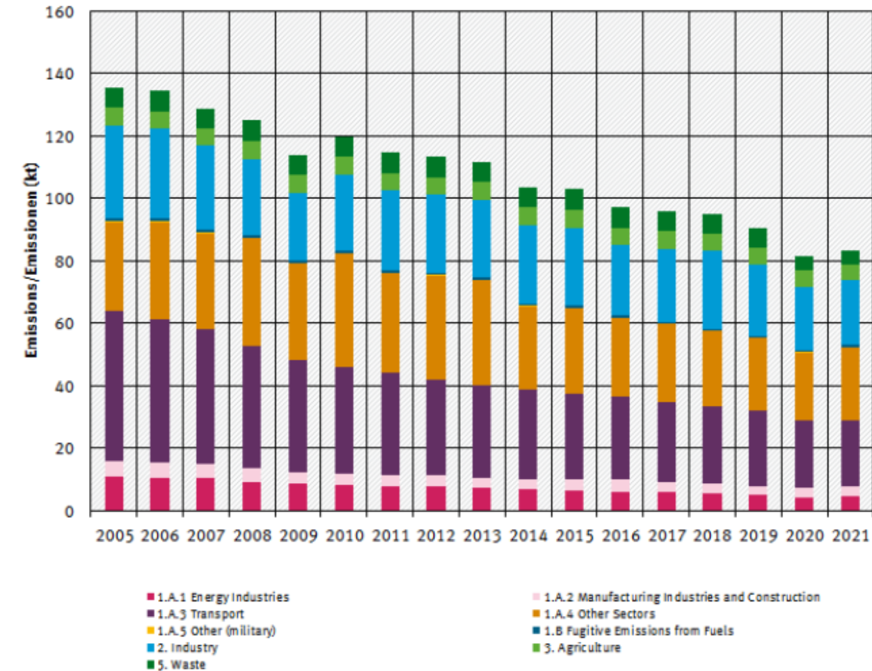
PM 2.5 trend by sector
