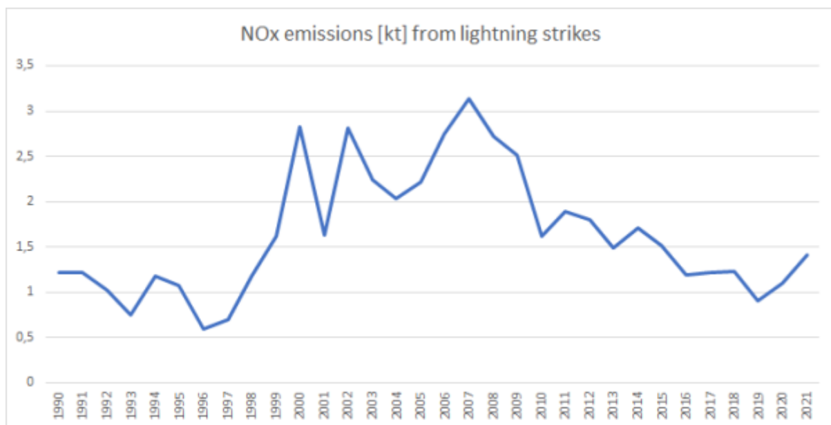
Figure 1: NFR 11.C, NO x emissions from lightning
