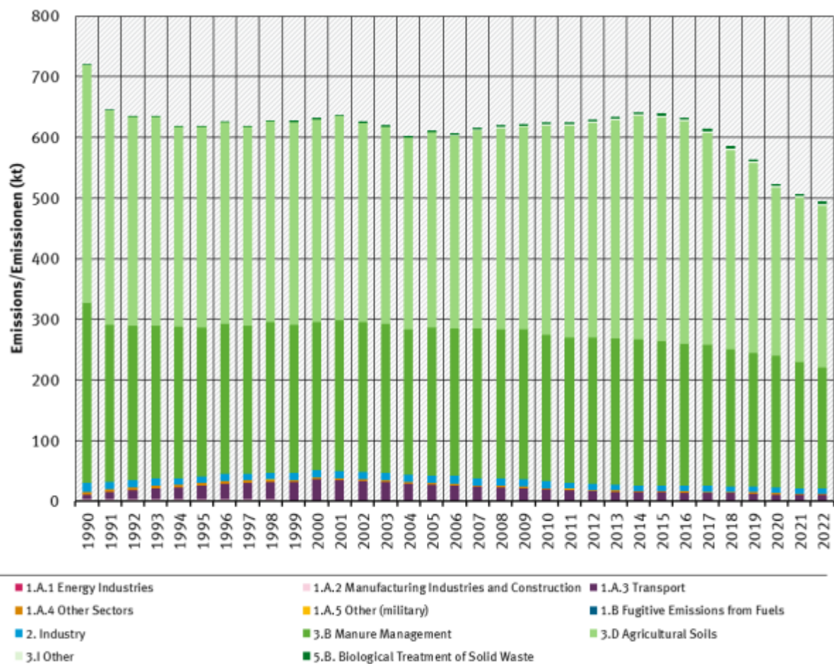
NH 3 trend by sector
