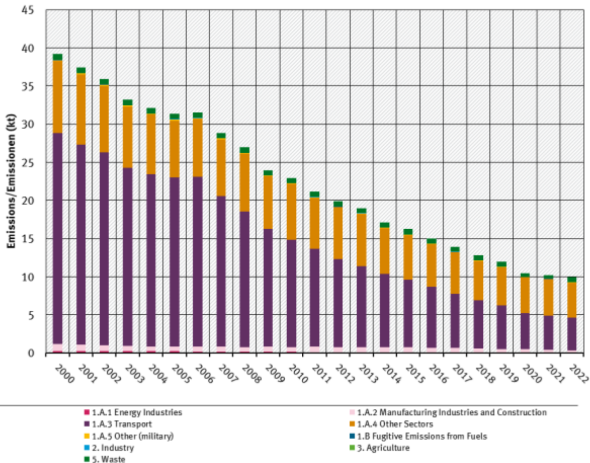
Black Carbon emissions from 2000 / Black Carbon Emissionen erst ab 2000
