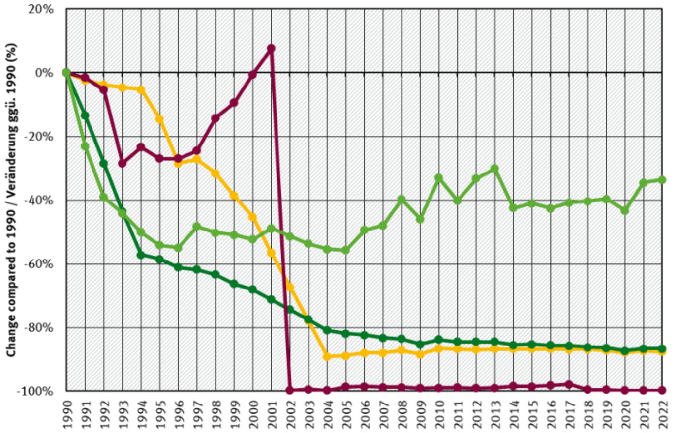
Legend: PCB (yellow line), Dioxine (Teq) (dark green line), HCB (maroon line), PAH Total (light green line)
