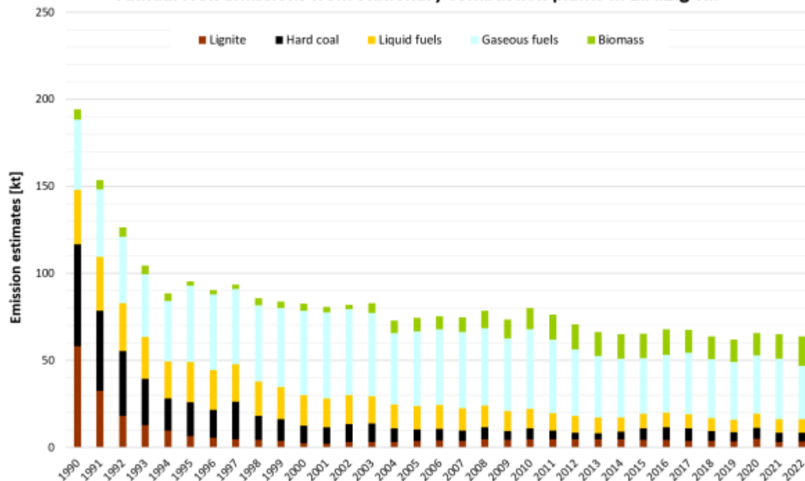
Annual NO x emissions from stationary combustion plants in 1.A.2.g viii
