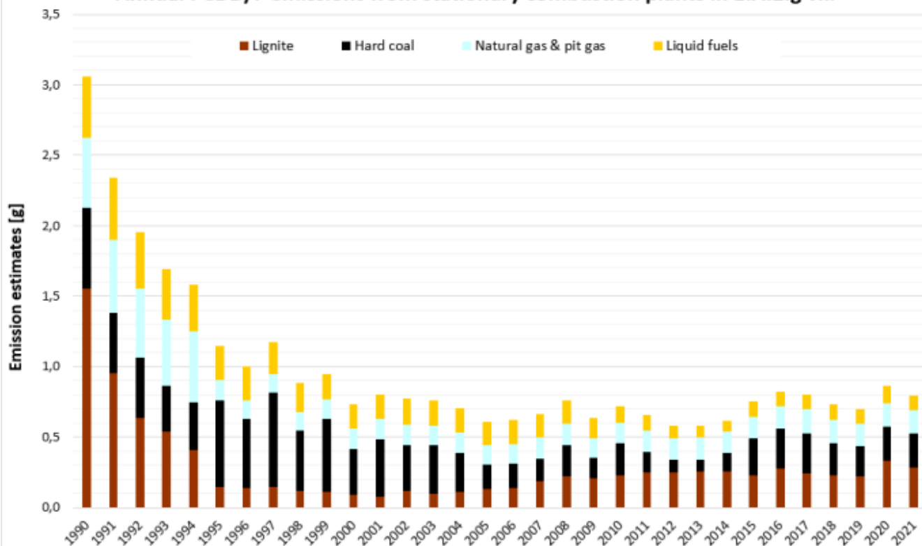
Annual PCDD/F emissions from stationary combustion plants in 1.A.2.g viii
