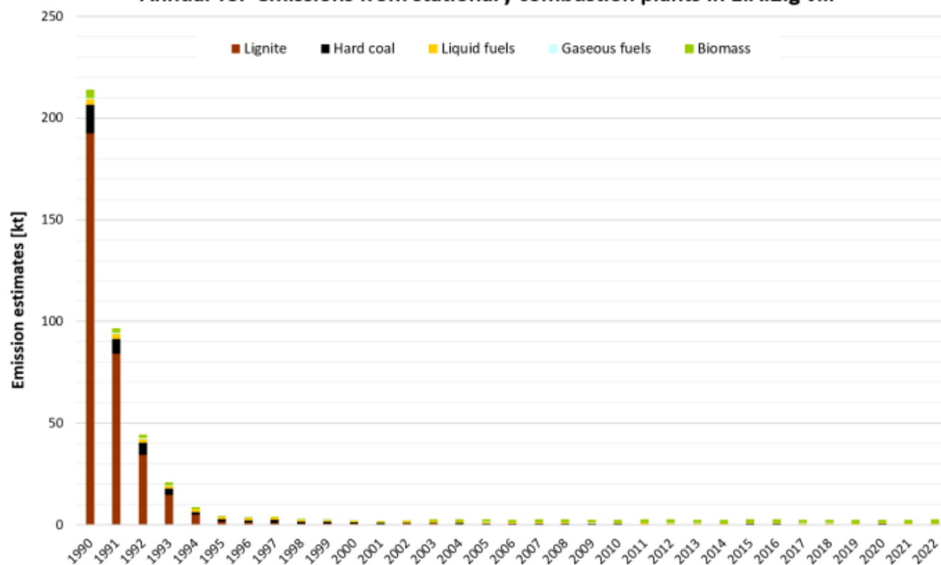
Annual TSP emissions from stationary combustion plants in 1.A.2.g viii
