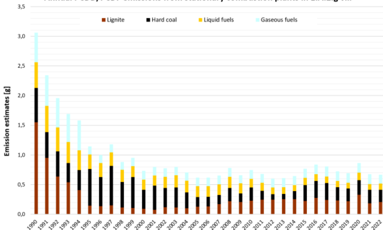
Annual PCDD/PCDF emissions from stationary combustion plants in 1.A.2.g viii
