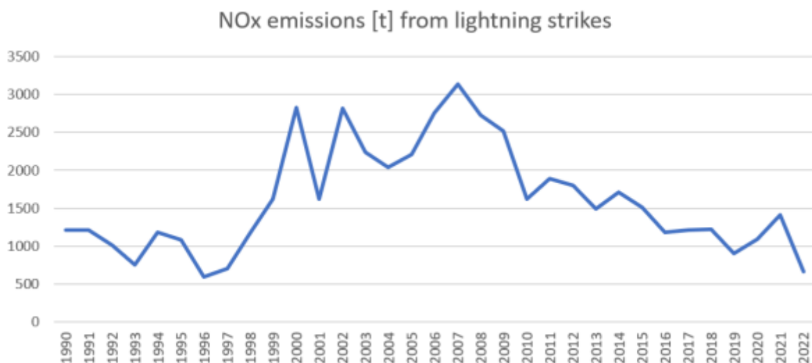
Figure 1: NFR 11.C, NO x emissions from lightning
