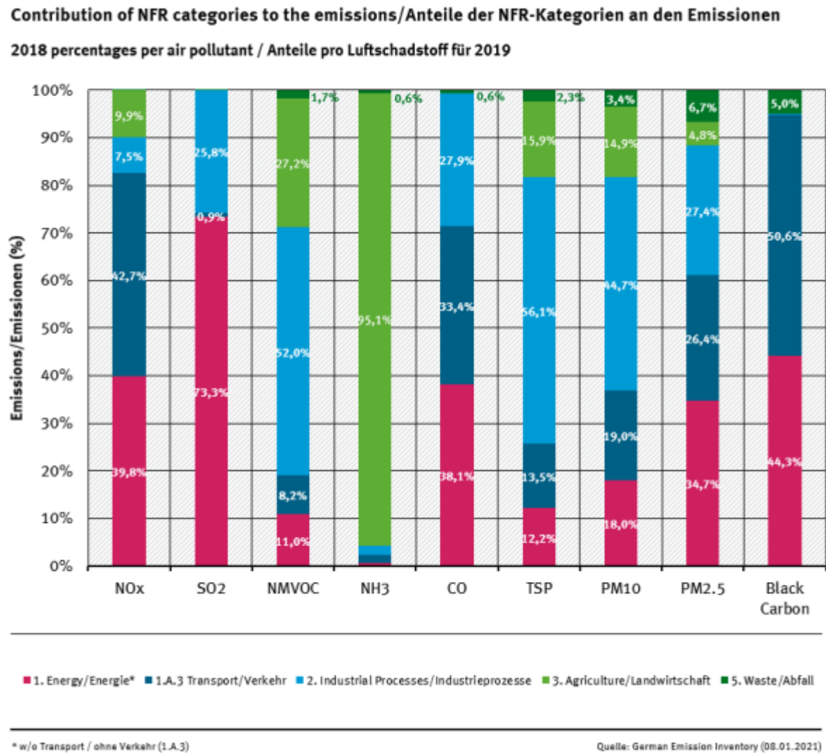
Contribution of NFR categories to the emissions
