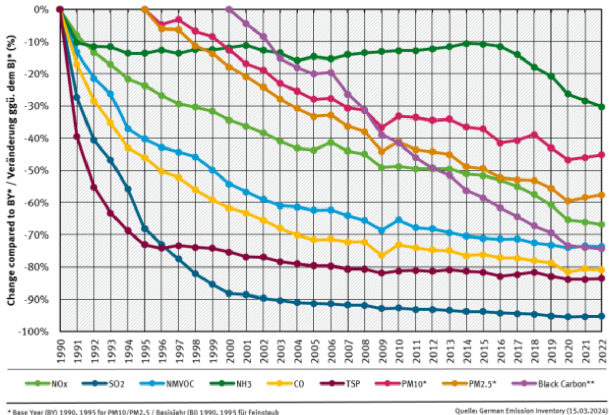
Total emission trends for the most important pollutants in percent decrease compared to a base year, set to 1995 for PM 2.5 and PM 10 , to 2000 for Black Carbon, and 1990 for all other pollutants.
