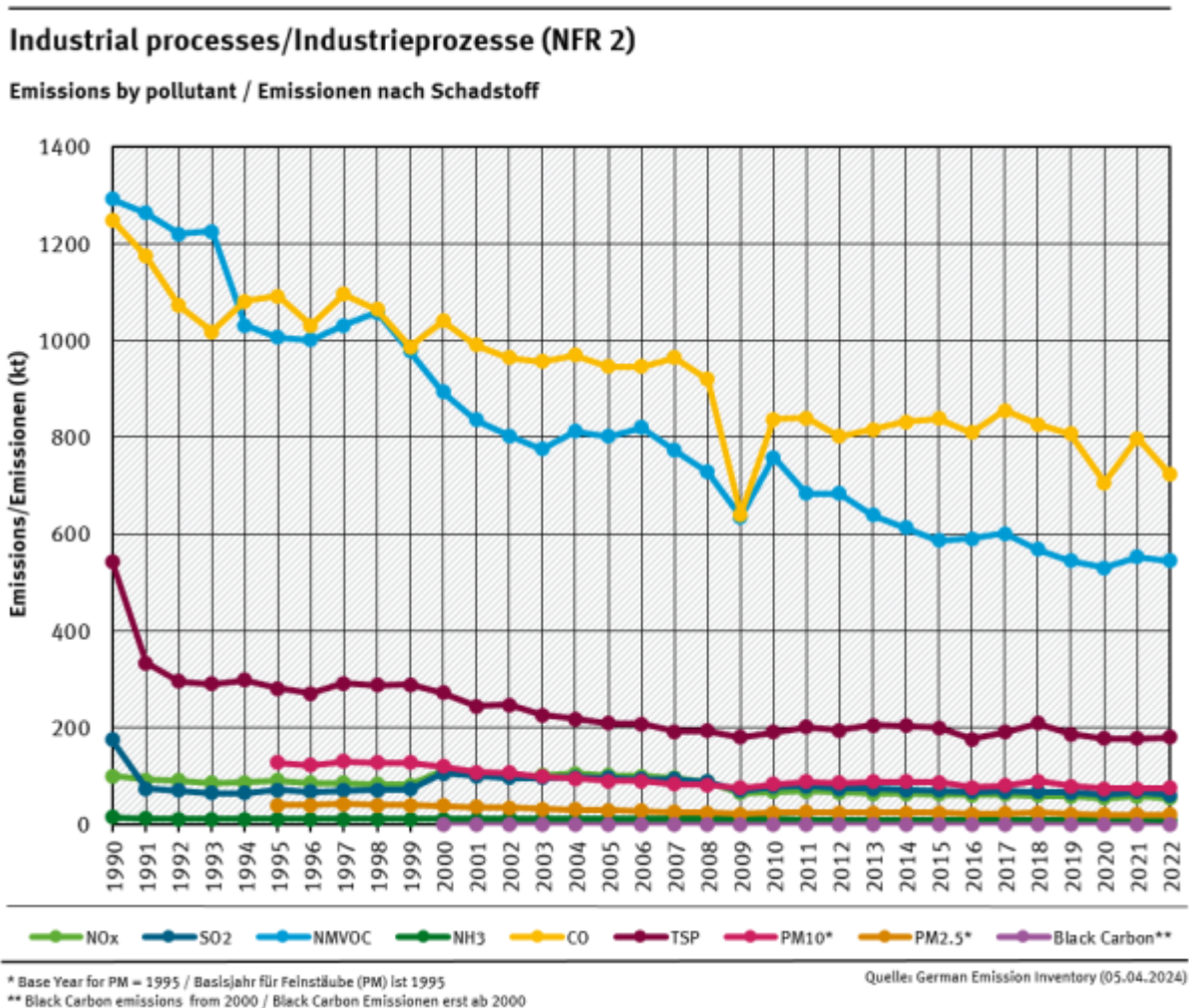
Chart showing emission trends for main pollutants in NFR 2 - Industrial Processes :
