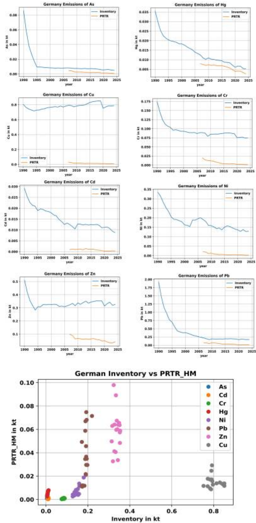
Figure 6: The upper images show yearly time series data for heavy metals extracted from the PRTR database plotted versus the reported inventory data of Germany. The lowermost image illustrates the correlation between each of the reported time-series with the respective HM species from the PRTR data.
