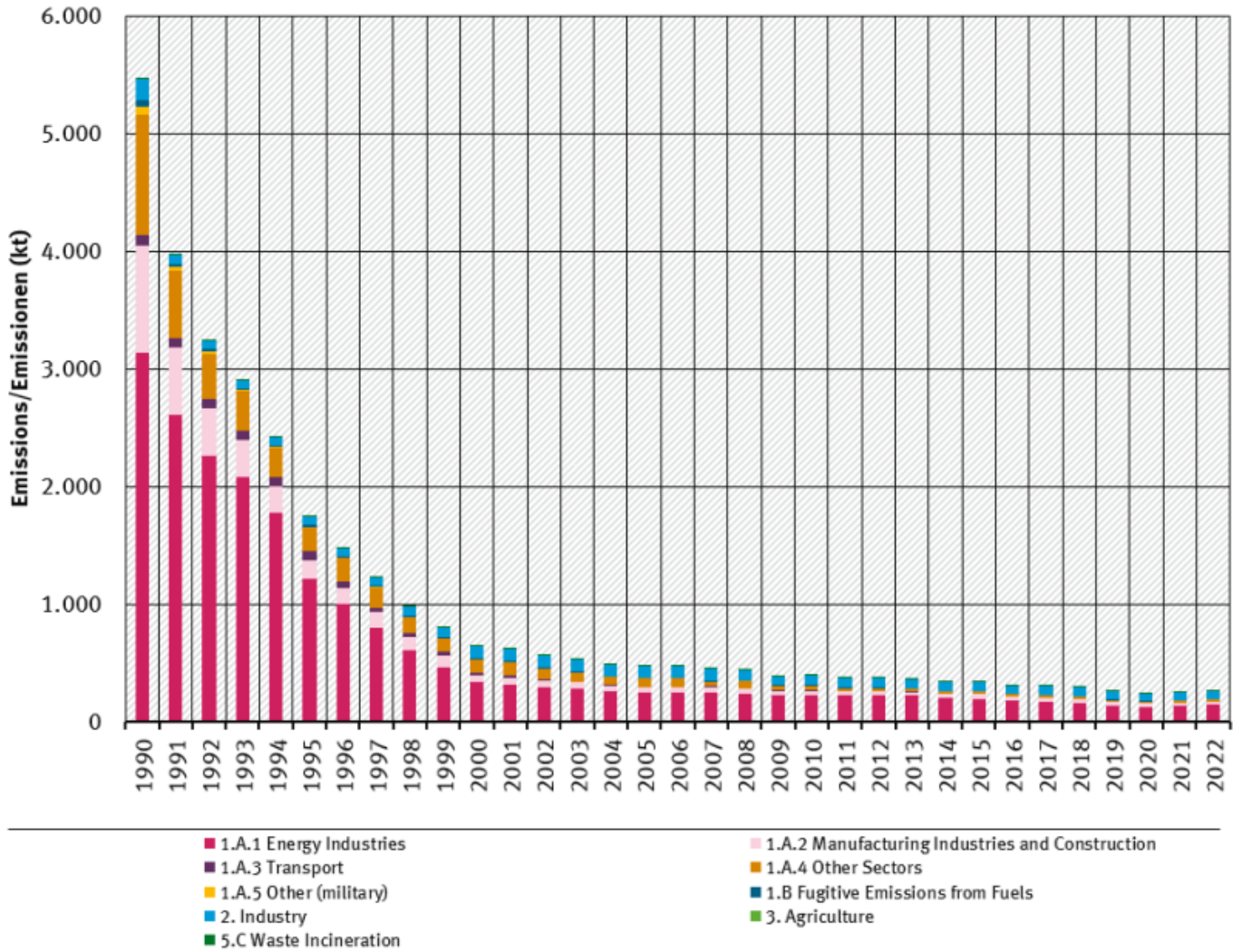
SO 2 trend by sector
