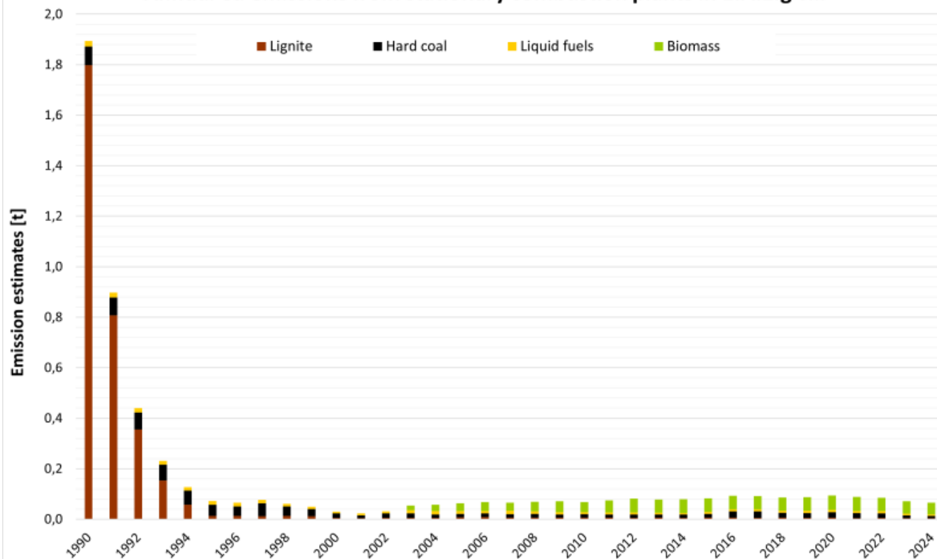
Annual Cd emissions from stationary combustion plants in 1.A.2.g viii
