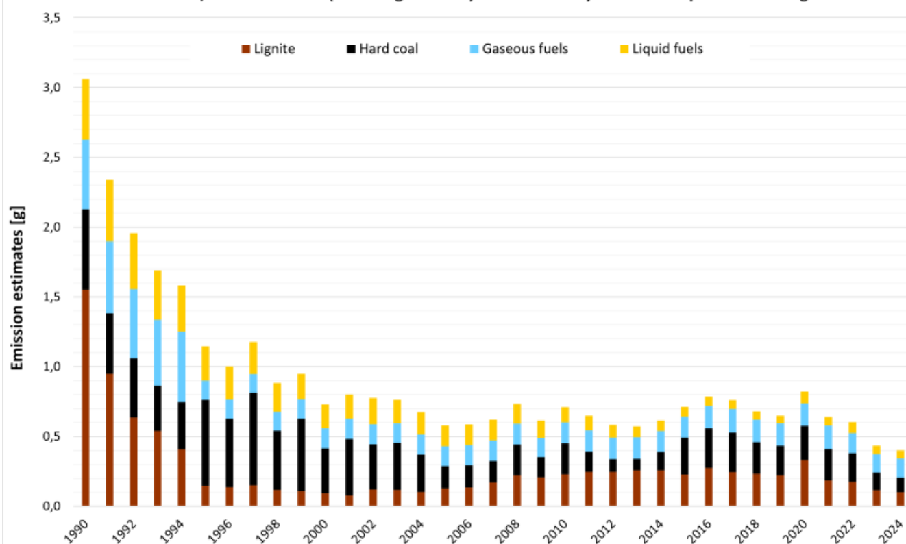
Annual PCDD/PCDF emissions (excluding biomass) from stationary combustion plants in 1.A.2.g viii
